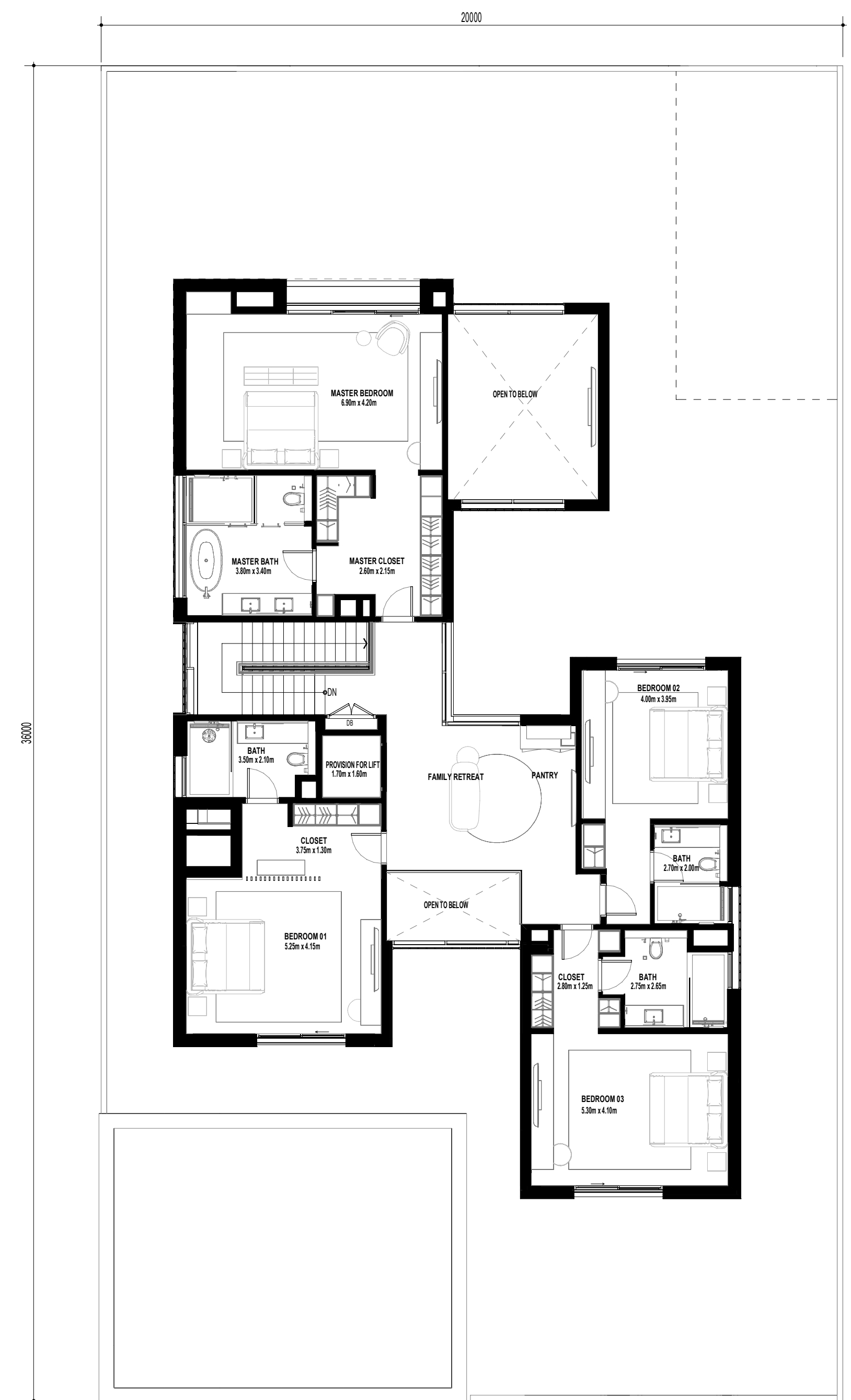
FIRST FLOOR
