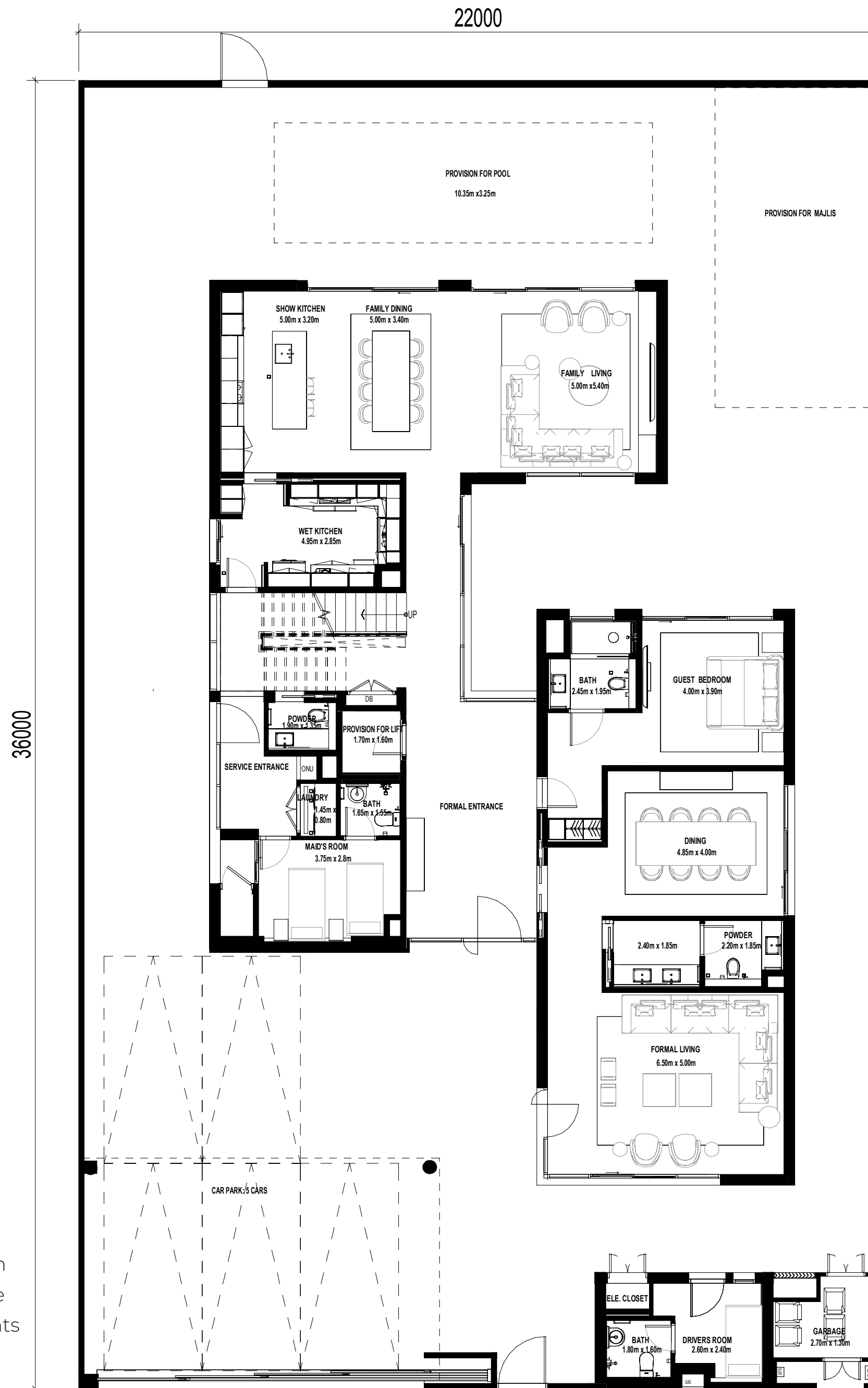
GROUND FLOOR
