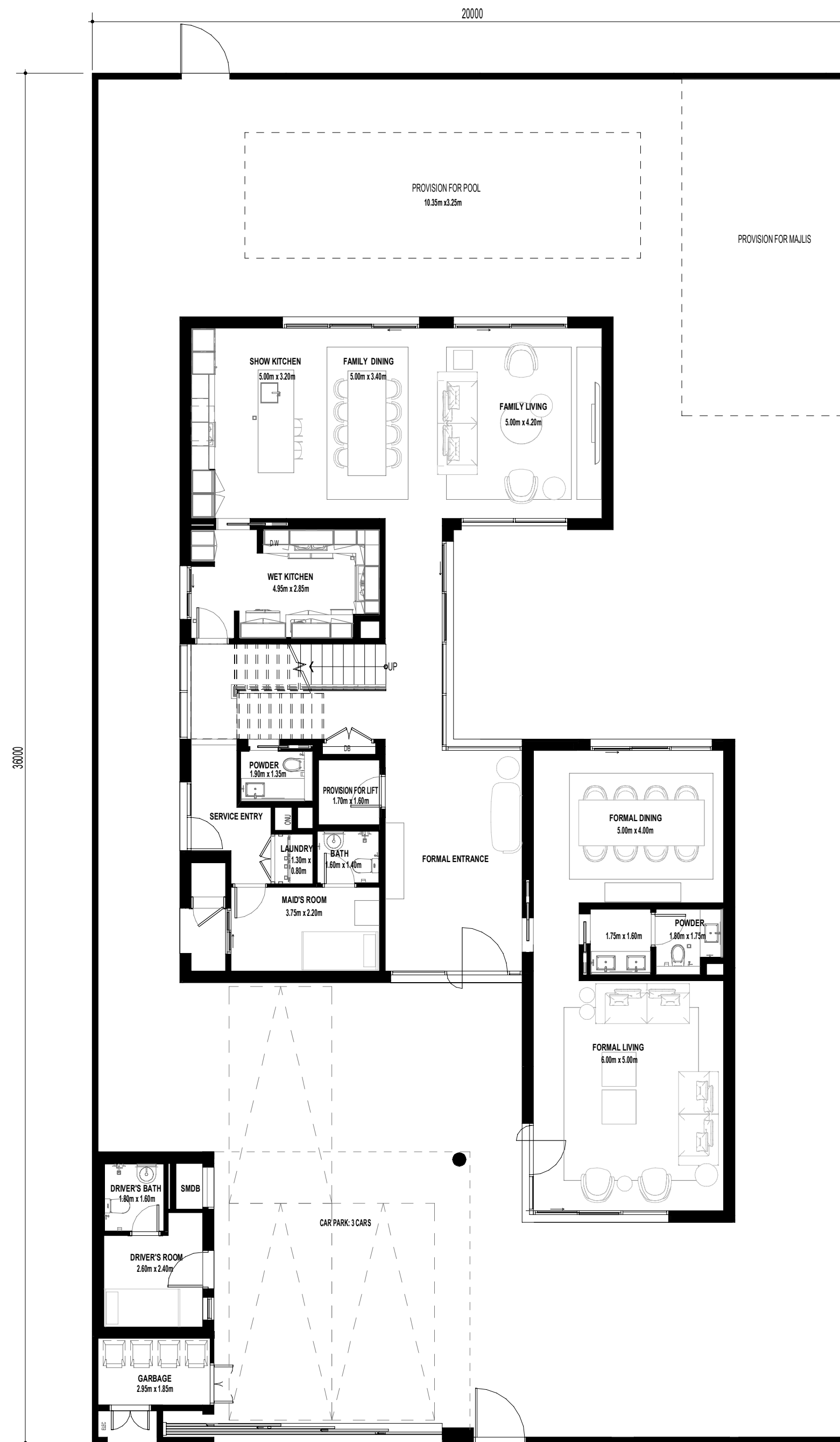
GROUND FLOOR
